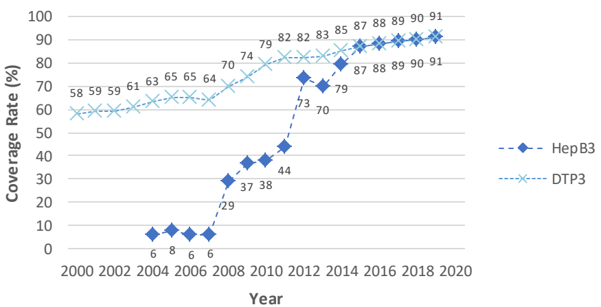
India: HepB3 vs. DTP3
