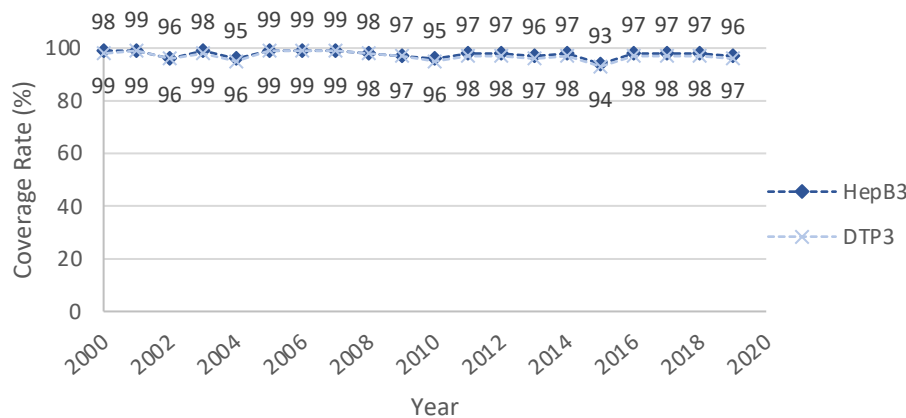
Saint Kitts and Nevis: HepB3 vs. DTP3
