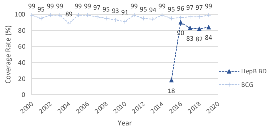
Saint Kitts and Nevis: HepB BD vs. BCG
